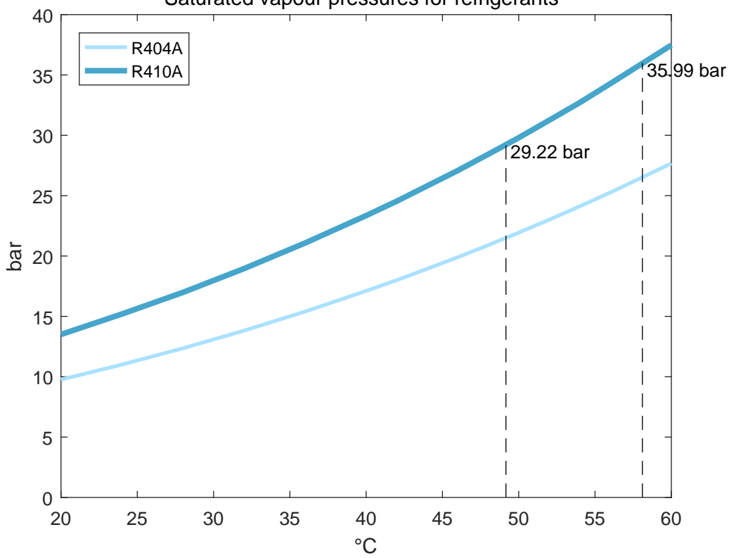
Saturated vapour pressures for refrigerants
