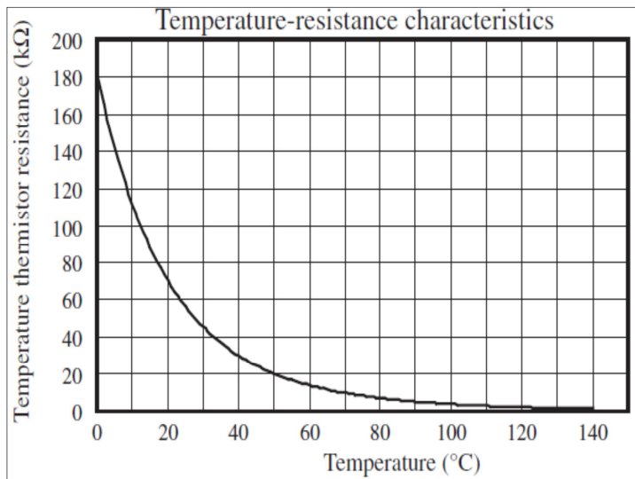
Power Transistor Thermistor (Tho-P)
