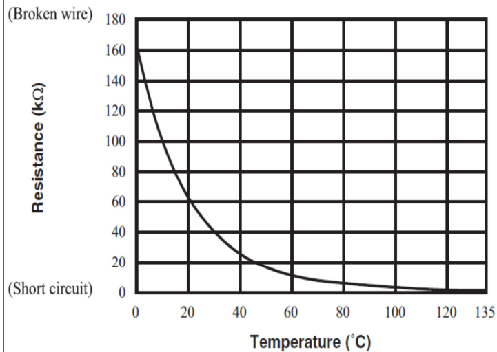
Discharge Pipe Thermistor (Tho-D)
